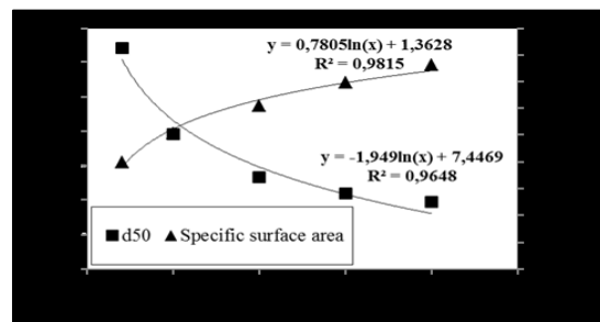
Figure 12. The influences of five different grinding times on d 50 size and specific surface area
