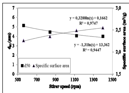
Figure 3. The influences of four different stirrer speeds on d_{50} size and specific surface area
