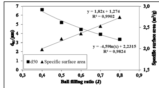
Figure 5. The influences of five different ball filling ratios on d_{50} size and specific surface area
