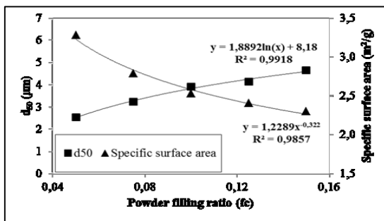
Figure 7. The influences of five different powder filling ratios on d_{50} size and specific surface area
