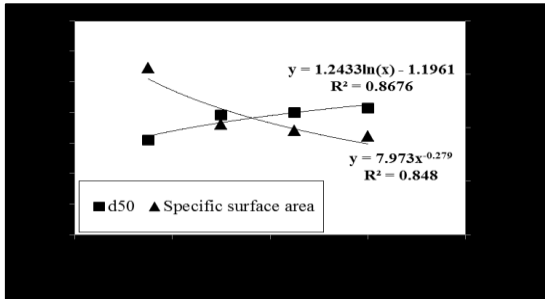
Figure 9. The influences of four different solid ratios on d 50 size and specific surface area
