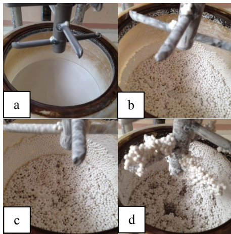
Figure 10. Images of wet grinding of calcite at different solid ratios (a: 35%, b: 50%, c: 65%, d: 80%)
