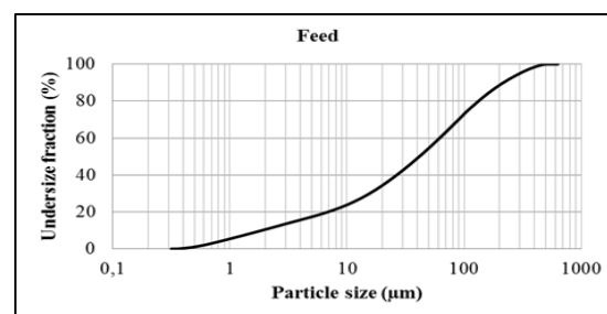
Figure 1. Feed size distributions of the calcite sample
