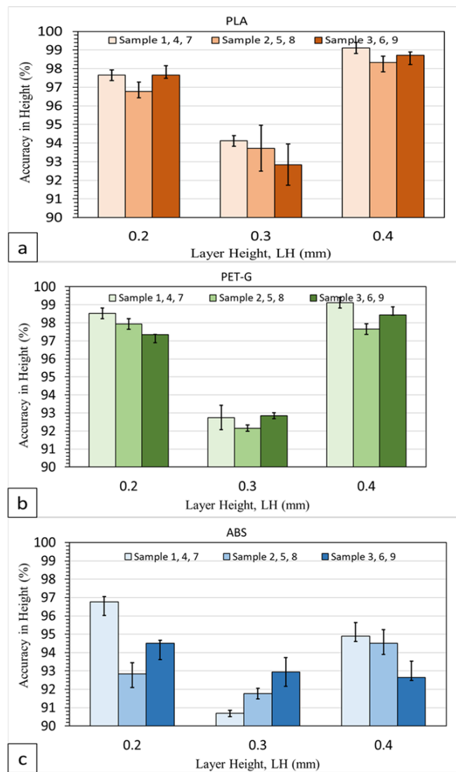
Figure 7. Accuracy values in height; PLA(a), PET- G(b) and ABS(c)
